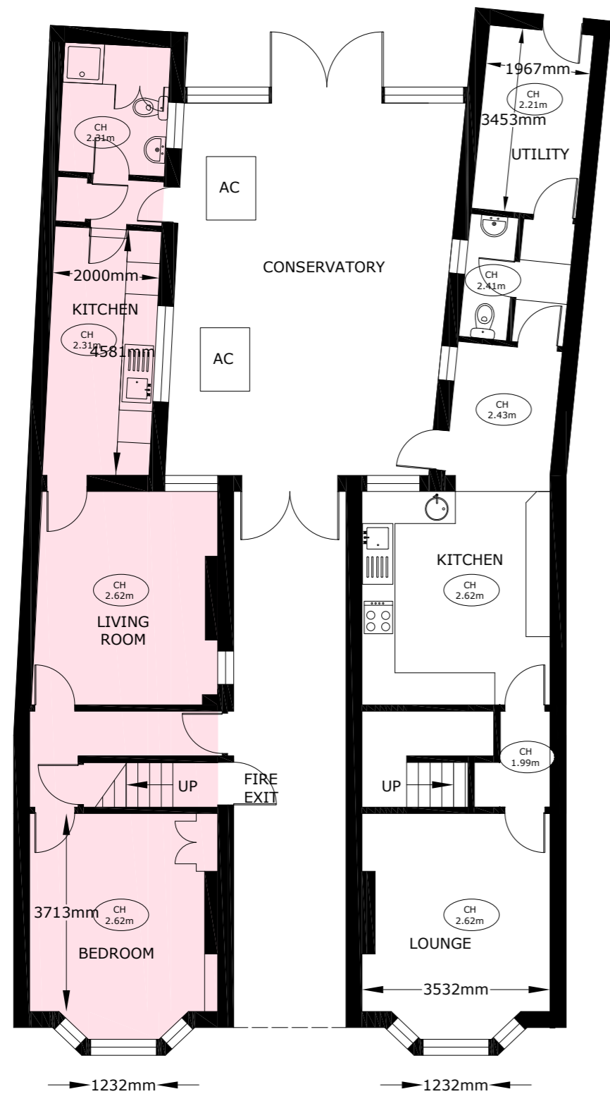
GROUND FLOOR
