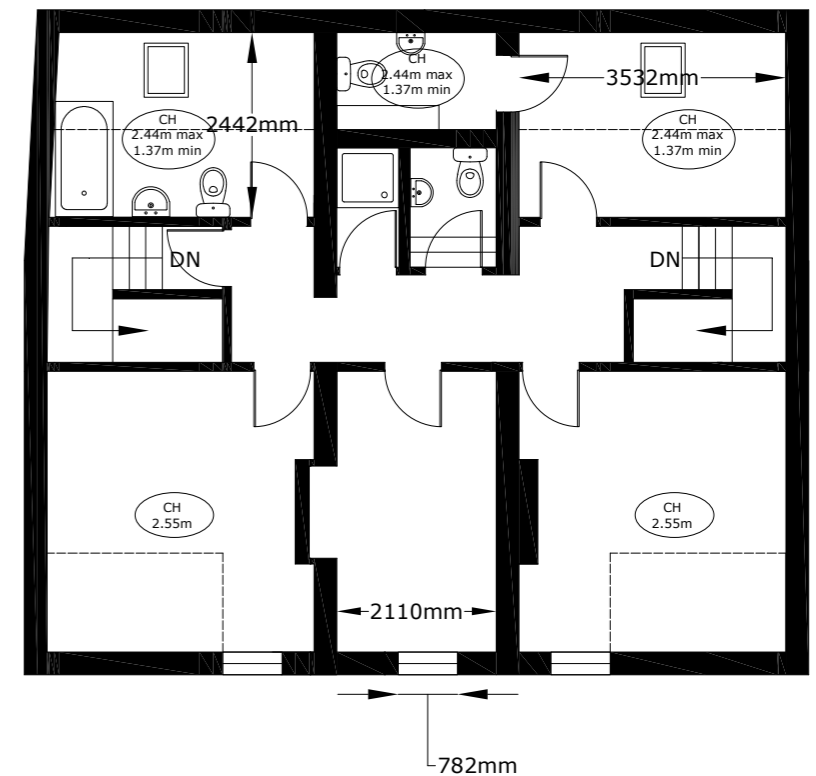
SECOND FLOOR
